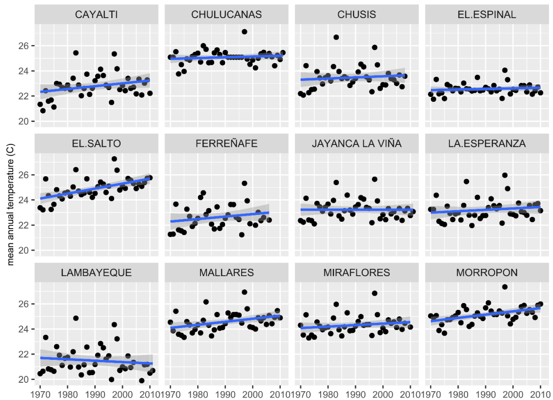
Supplementary Figure 1. Time series of mean annual temperature for 12 weather stations of northern Peru.
