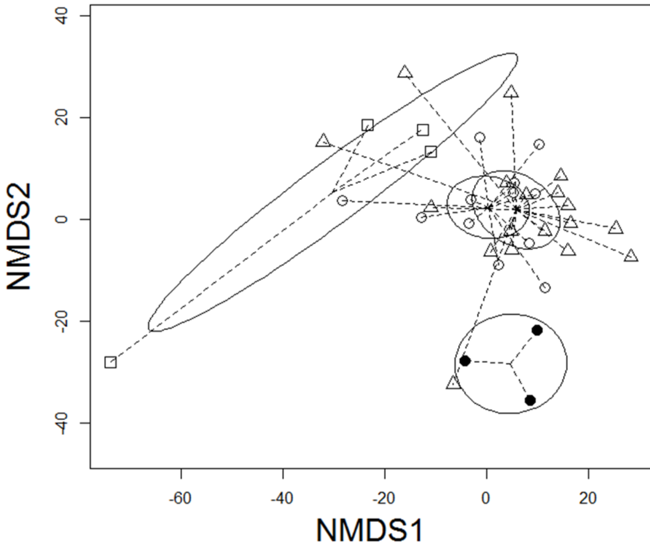
Figure 3. Non-metric multidimensional scaling ordination (NMDS) of microhabitat plots of antpittas in the Llavivuco Valley, Cajas National Park. Species' symbols represent: \Delta = Rufous Antpitta ( Grallaria rufula ); \circ = Chesnut-crowned Antpitta ( Grallaria ruficapilla ); \bullet = Undulated Antpitta ( Grallaria squamigera ); \square = Tawny Antpitta ( Grallaria quitensis ). The stress value of the NMDS was 0.03.
