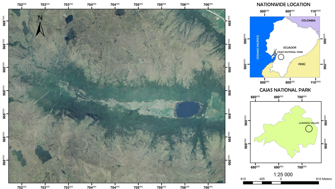
Figure 1. Study area showing the location of the Llaviucu Valley, Cajas National Park, southern Ecuador.
